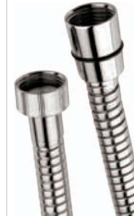
CODE:KL-FH10001S ■ BRASS FLEXIBLE HOSE, SINGLE LOCK 1/2"F*1/2"F
